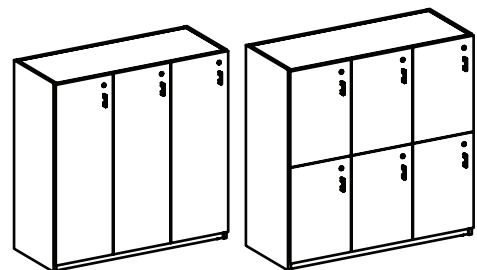
3-cluster
